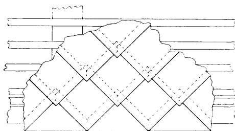
Fig. 13. Diagonal Skiferdækning.
